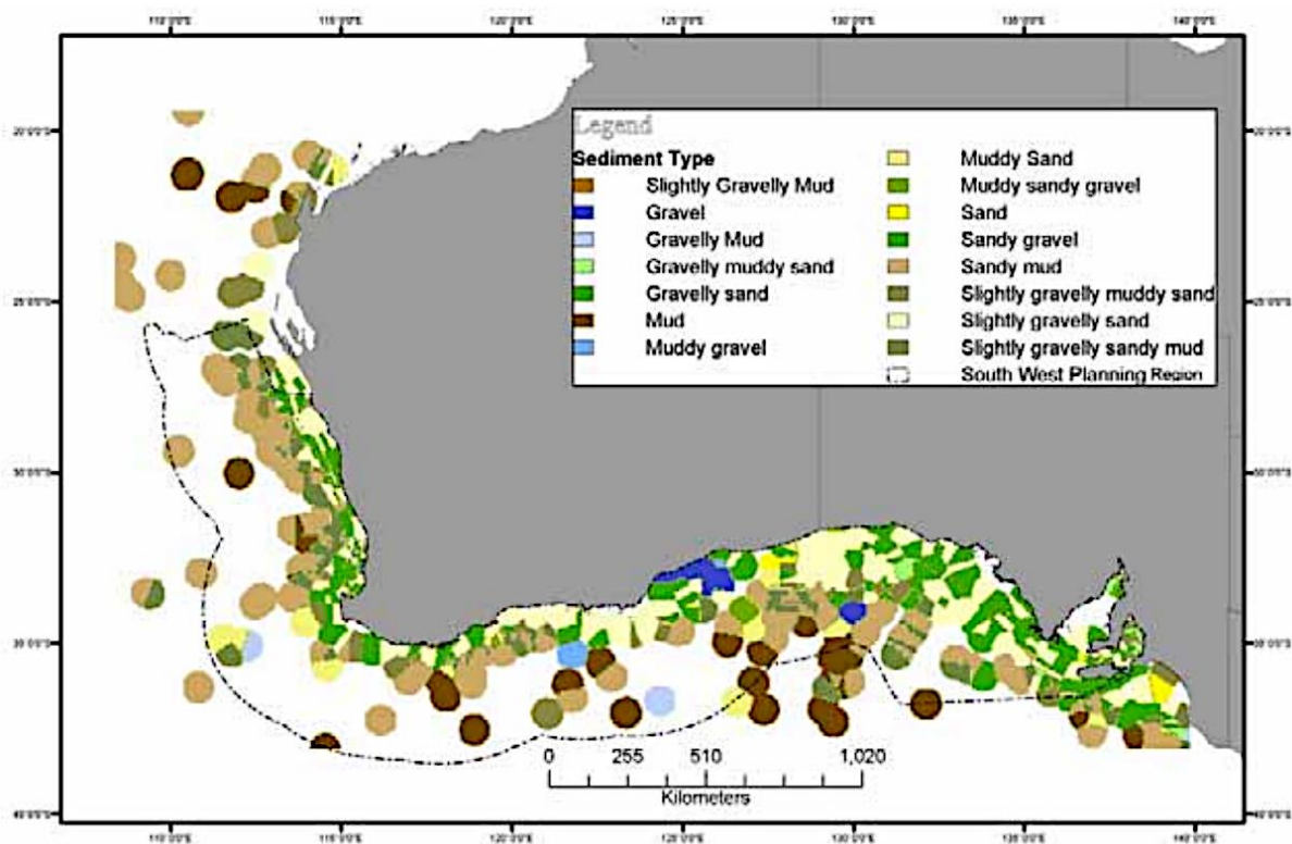
Figure 5-15 Map showing the Folk Classification of seabed sediments in the southwest planning region. Source Potter et al. (2006)
